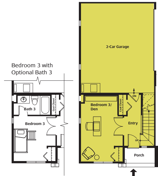
Erica (E) Lower Floor Plan
